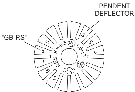
Figure 41 GB-RS, K=4.3, Pendant CENTRAL
