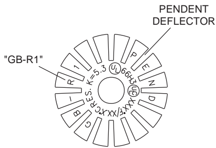
Figure 39 GB-R1, K=5.3, Pendant CENTRAL
