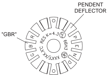
Figure 35 GBR, K=4.3, Pendent CENTRAL
