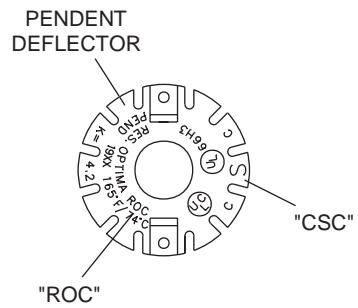
Figure 44 ROC, K=4.2, Concealed Pendent CENTRAL
