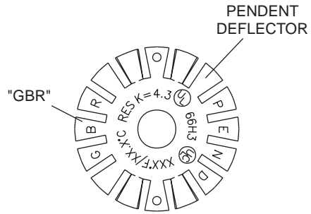
Figure 36 GBR, K=4.3, Concealed Pendent CENTRAL
