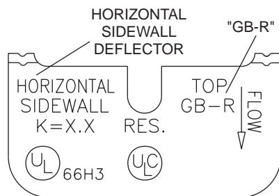
Figure 38 GB-R, K=5.4, Horizontal Sidewall CENTRAL
