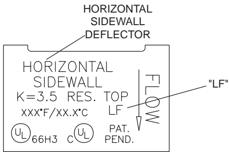
Figure 43 LF, K=3.5, Horizontal Sidewall CENTRAL
