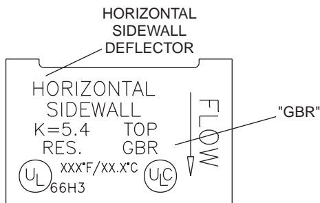
Figure 37 GBR, K=5.4, Horizontal Sidewall CENTRAL
