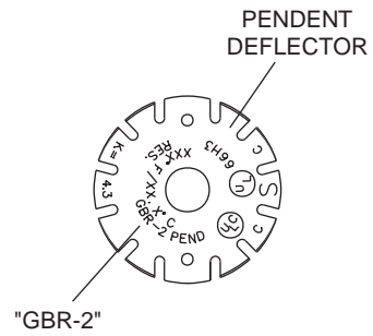
Figure 40 GBR-2, K=4.3, Pendant CENTRAL
