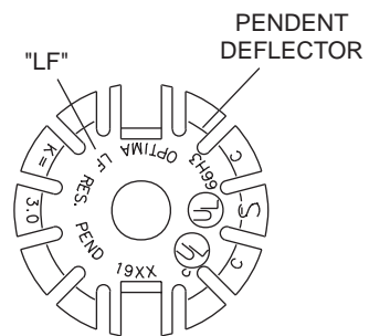
Figure 42 LF, K=3.0, Pendant CENTRAL
